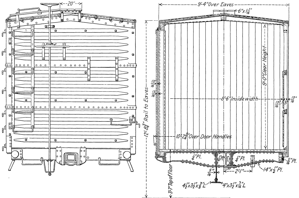
Fig. 2852—Cross-Section and End of 40-Ton Box Car Shown in Figs. 2849, 2853 and 2854.
