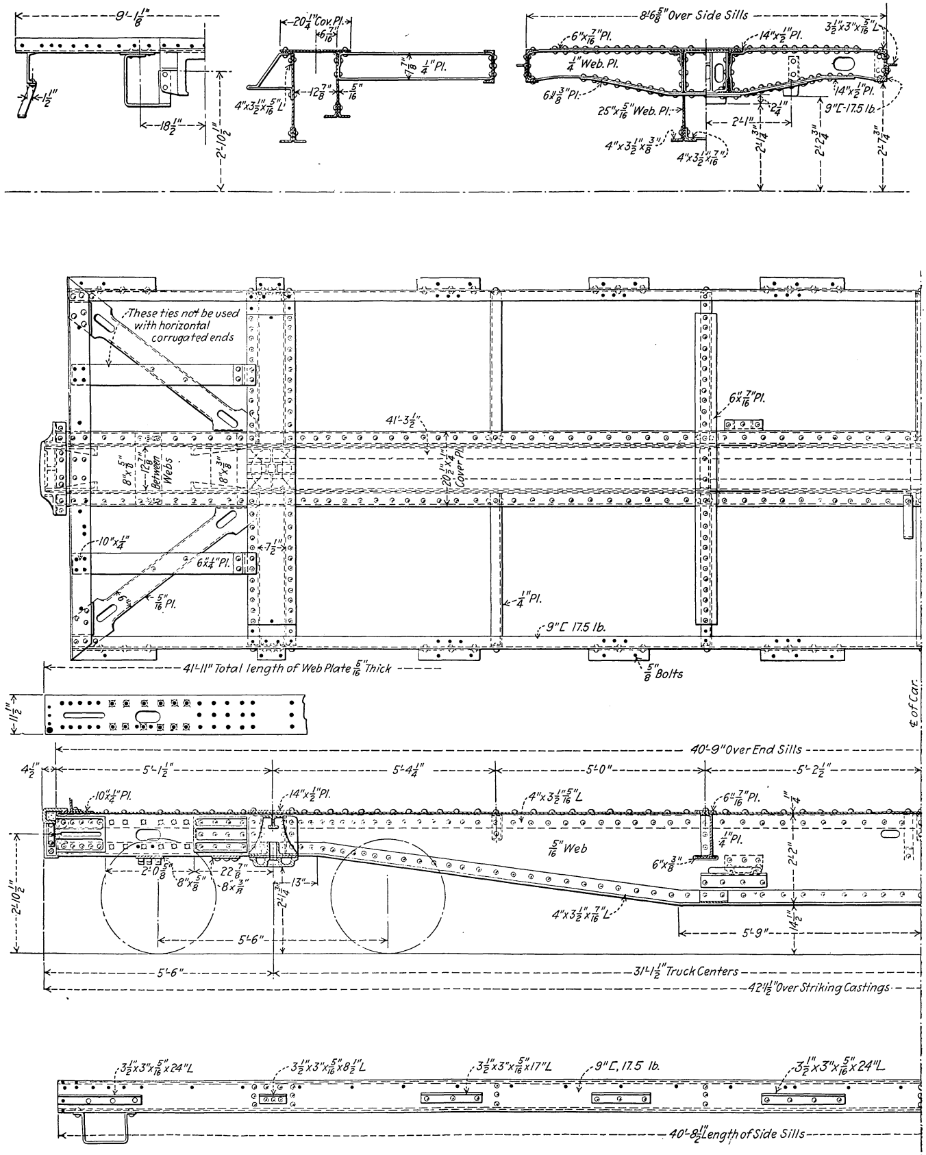
Fig. 2854—Steel Underframe for 40-Ton Double Sheathed Box Car Shown in Figs. 2849, 2852 and 2853.
